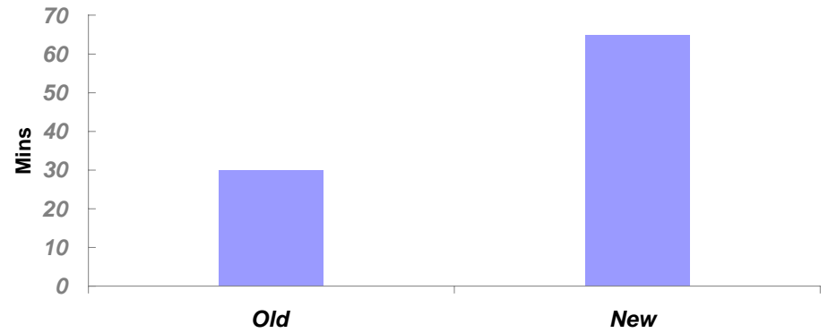
Cumulative Stock Removal FLX115060 Manual Test on Mild Steel
